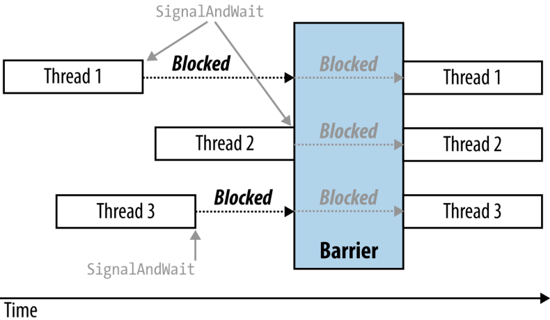
Figure 22-3. Barrier
