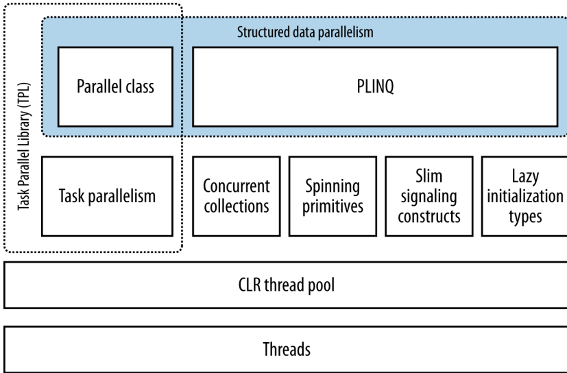
Figure 23-1. PFX components
