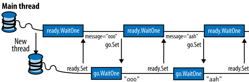
Figure 22-2. Two-way signaling
