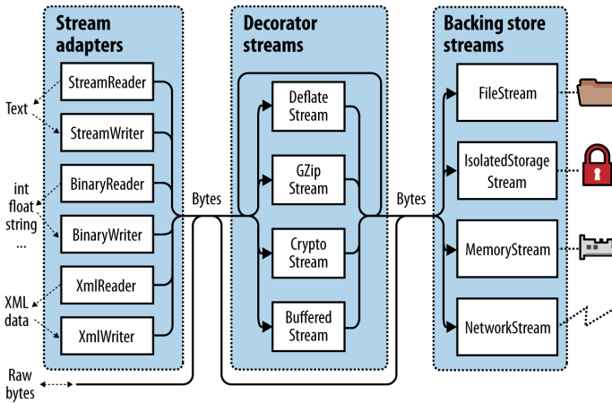
Figure 15-1. Stream architecture
