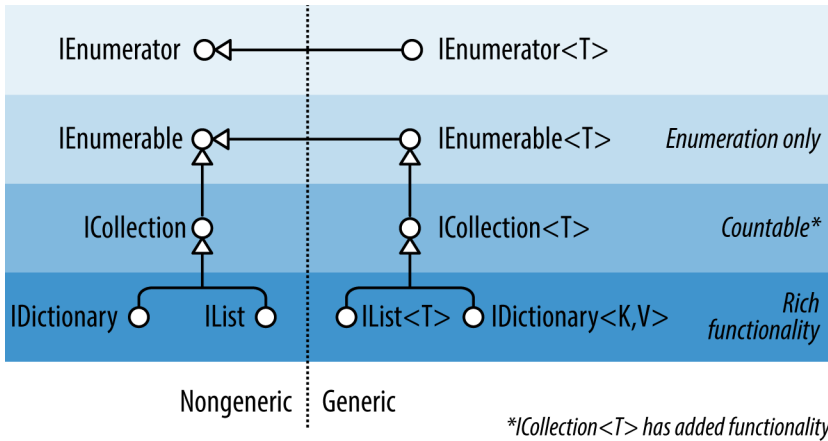
Figure 7-1. Collection interfaces
