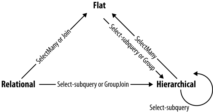
Figure 9-1. Shape-changing operators
