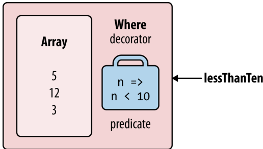
Figure 8-3. Decorator sequence
