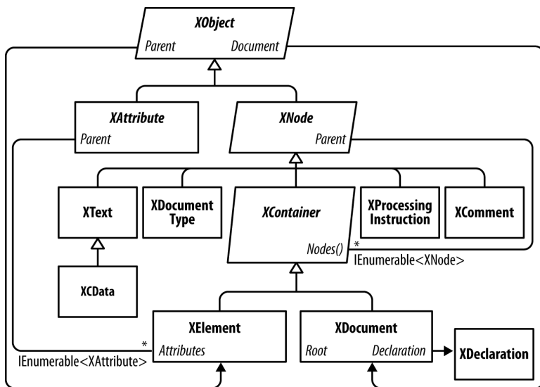
Figure 10-1. Core X-DOM types
