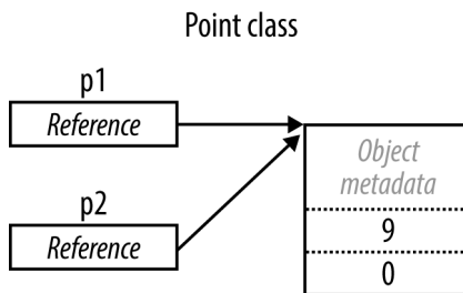
Figure 2-4. Assignment copies a reference
