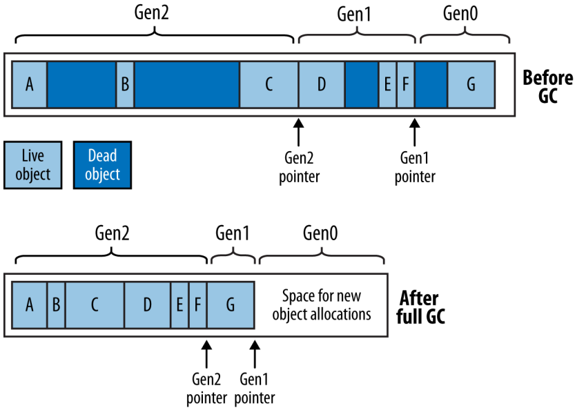
Figure 12-2. Heap generations
