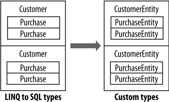
Figure 9-2. Projecting an object hierarchy
