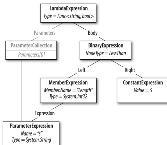
Figure 8-11. Expression tree
