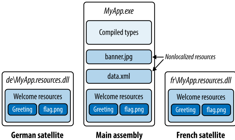
Figure 18-4. Resources
