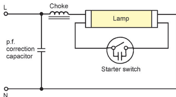
Figure 3.18 Fluorescent lamp circuit arrangements.
