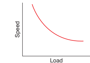
Figure 3.22 Series motor connections and characteristics.
